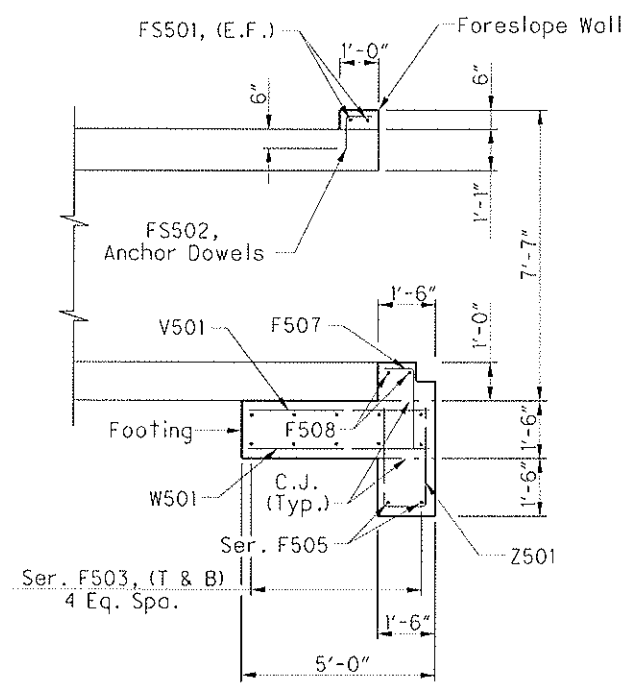
SECTION D-D CULVERT OUTLET BEVEL SHOWN
