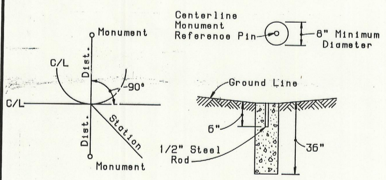
DETAIL FOR SETTING MONUMENTS
