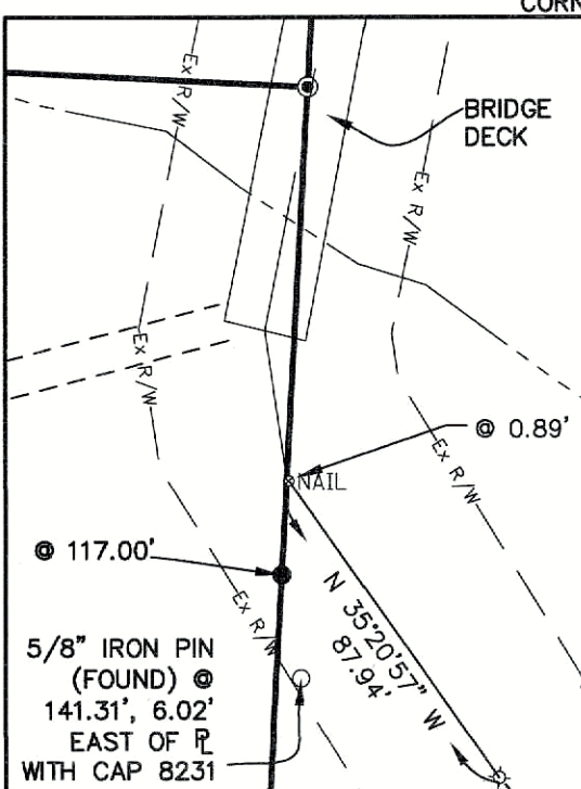
DETAIL "A" 1" = 50'
